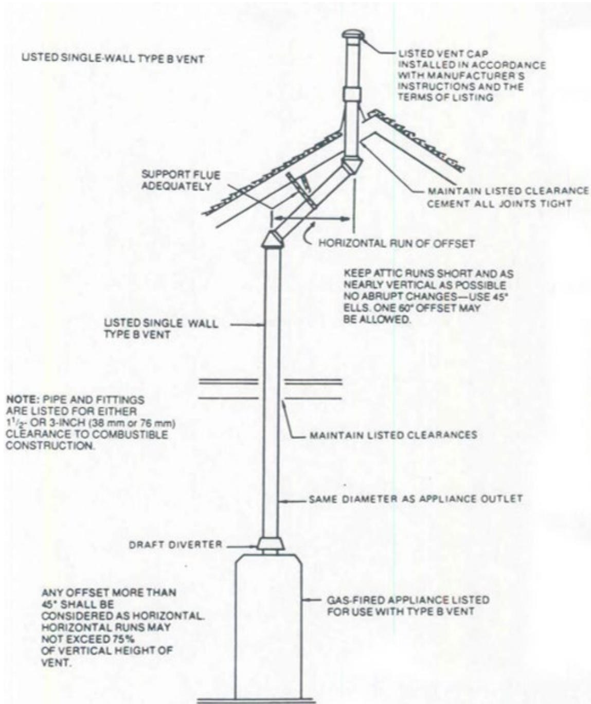
TYPICAL DETAILS FOR INSTALLATION OF SINGLE WALL NONMETALLIC TYPE B VENTS
