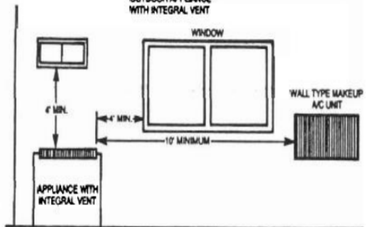
OUTDOOR VENT TERMINATION—APPLIANCES WITH INTEGRAL VENTS
