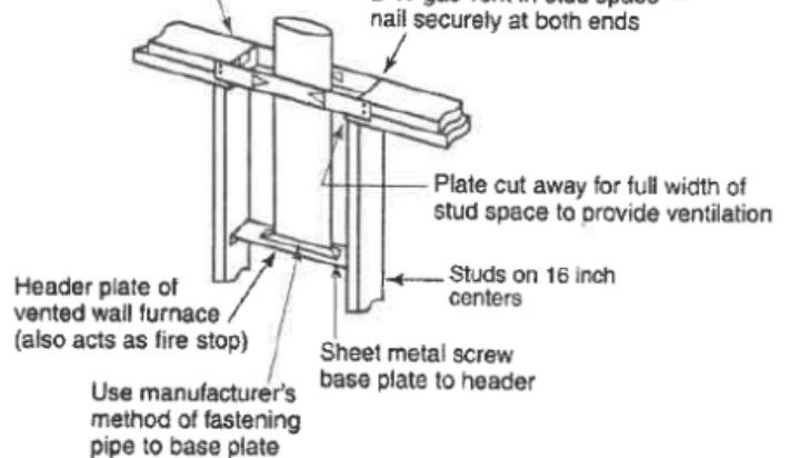
FIGURE 907.1 INSTALLATION OF TYPE B-W GAS VENTS FOR VENTED WALL FURNACES [NFPA 54: FIGURE 10.27.1.3]
